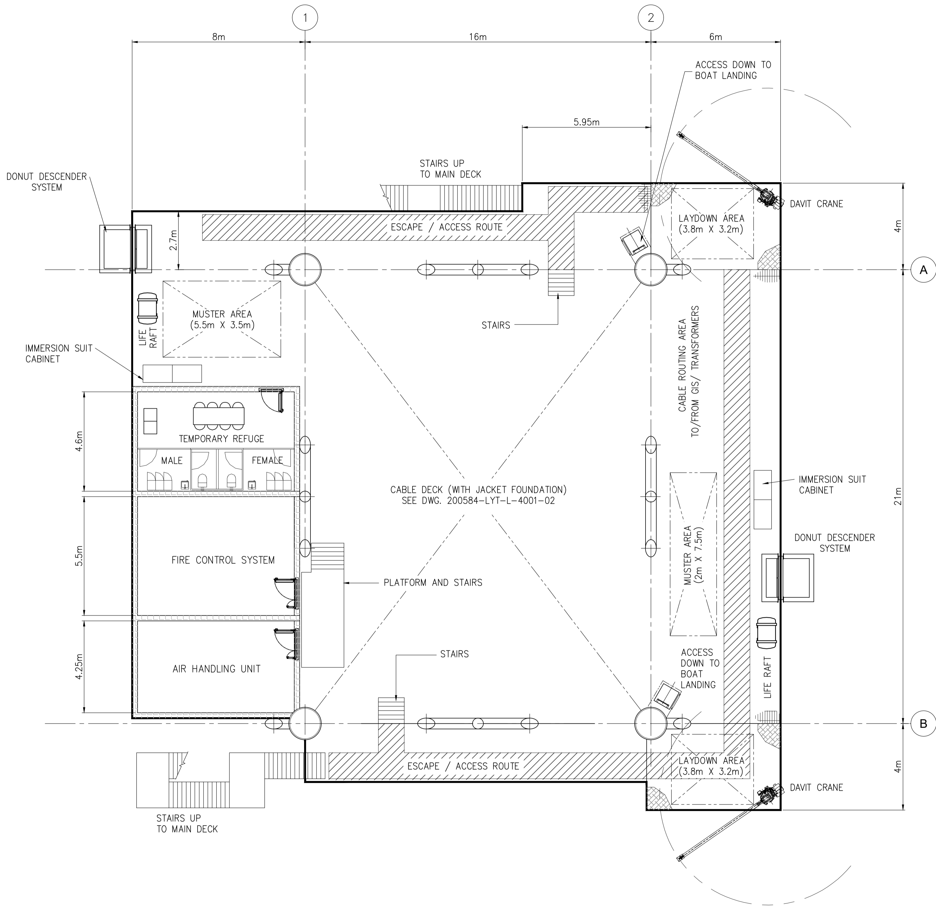
CELLAR DECK @ TOS. EL. + 17.100 (RELATIVE TO LAT)
